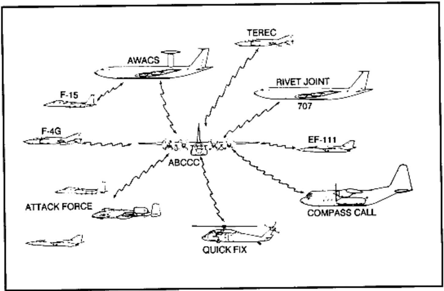
Figure 10-17. ABCCC control of EW assets.
